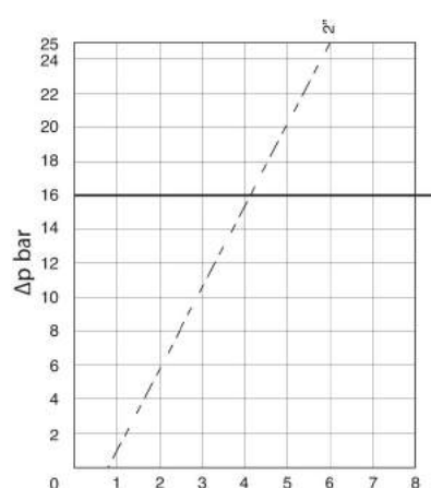
diagramma 15 diagram 15 testa head Ø90
