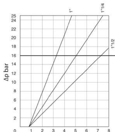
diagramma 13 diagram 13 testa head Ø50
