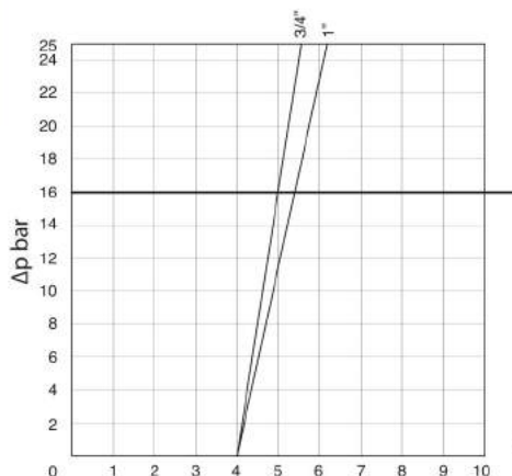
diagramma 1 diagram 1 testa head Ø40-Ø50
