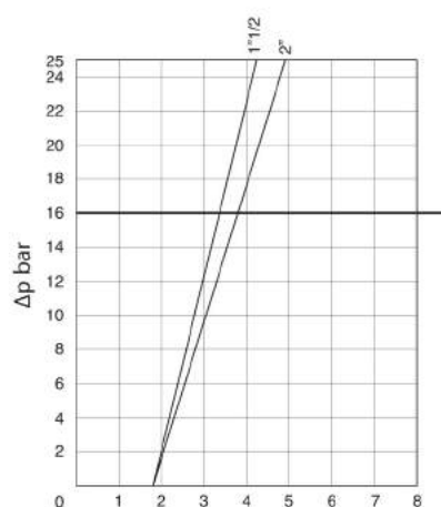
diagramma 7 diagram 7 testa head Ø90
